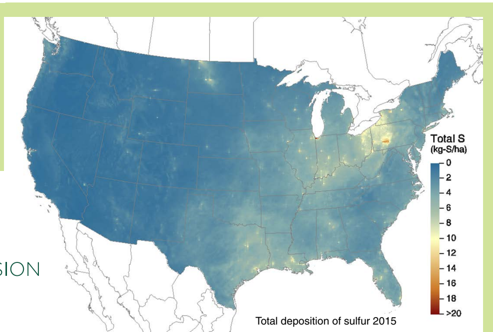
Figure 1. National atmospheric deposition map of total S in kilograms of S per hectare. To convert to pounds of S per acre, multiply the scale by 0.87. (U.S. Environmental Protection Agency image)
